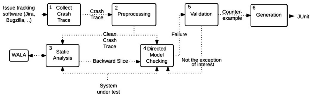
Figure 5. Overview of JCHARMING.
