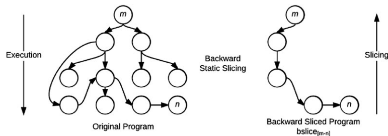
Figure 8. Hypothetical example of backward static program slicing.
