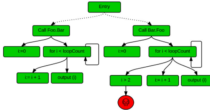
Figure 3. A toy program under model checking.
