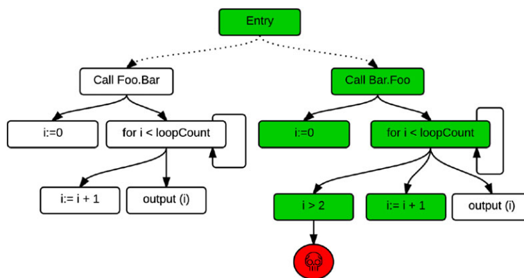
Figure 2. A toy program under testing.
