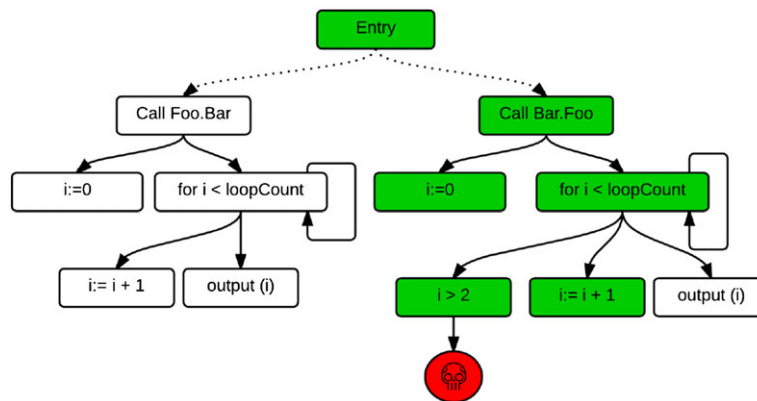
Figure 4. A toy program under directed model checking.
