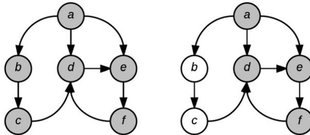
Figure 9. Hypothetical example representing bslice_{[a \leftarrow d]} (left) versus \bigcup_{i=d}^a bslice_{[f_{i+1} \leftarrow f_i]} (right) for a crash trace T = \{d, f, e\} .
