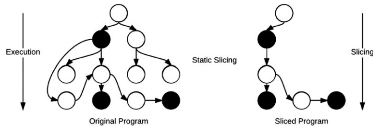
Figure 7. Hypothetical example of static program slicing.
