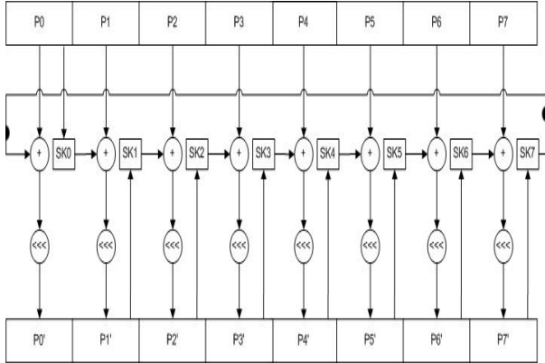
Figure 1: Round function of TREYFER, where SK_i(x) = \text{sbox}((x + K_i) \bmod 256)
