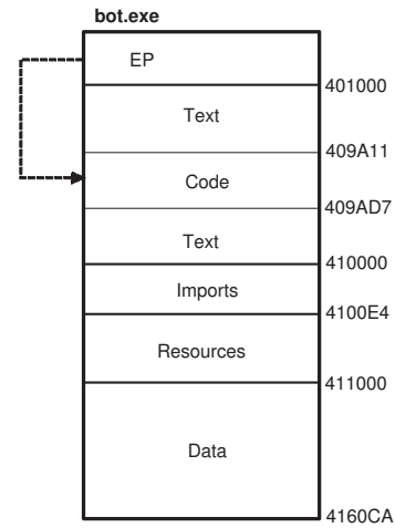
Fig. 2. Segments of the bot.exe binary file
