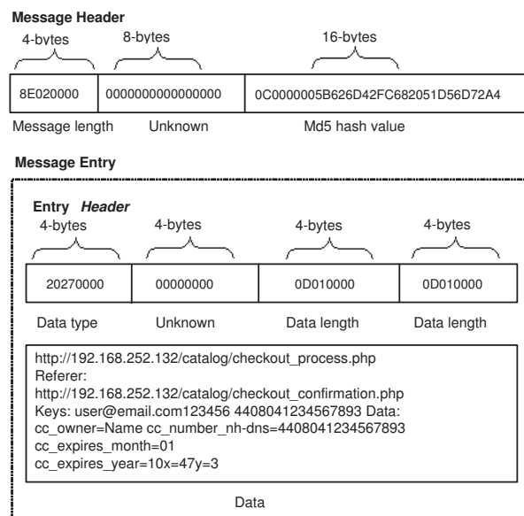
Fig. 7. A decrypted sample message
