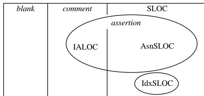
Figure 3. Categorization of Eiffel LOC
