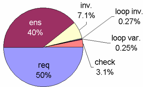
Figure 6. Distribution of assertions by kind (all project categories)
