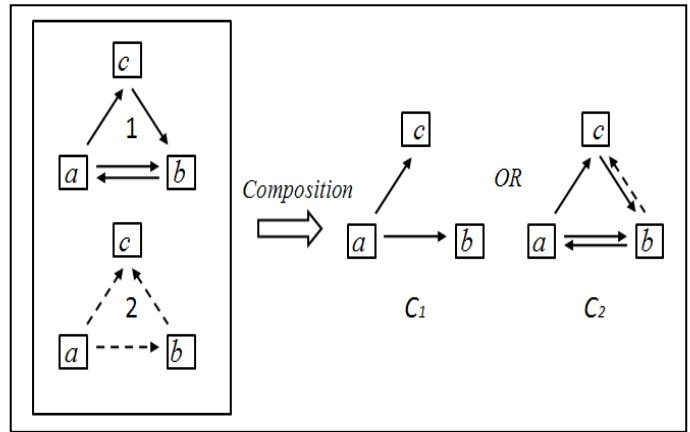
Figure 4. The composition of two initial agents’ action graphs through conjunction ( C_1 ) or adjunction ( C_2 ). As can be seen in C_1 emphasizes are on common paths within the two action graphs, while in C_2 the focus is on sum of the available paths.
