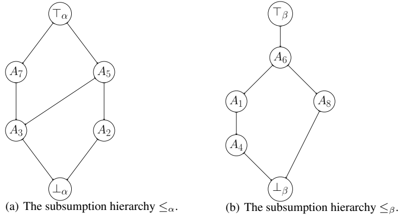
Fig. 2. The subsumption hierarchy over divisions.
