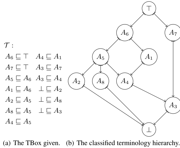
Fig. 1. An example ontology.
