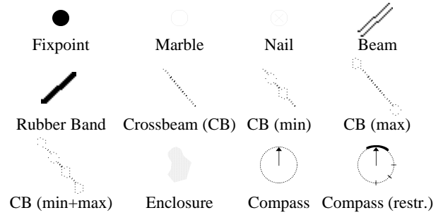
Figure 1: Basic language elements of VISCO
