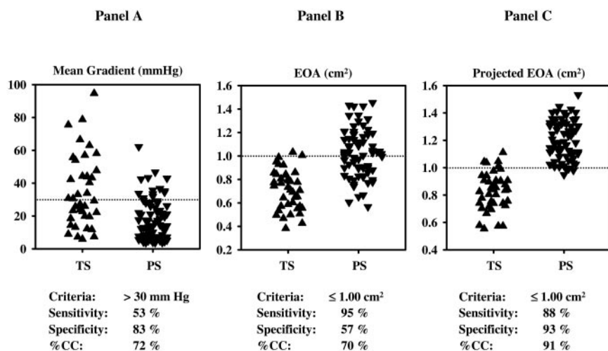
Figure 3. Distribution of mean gradient (A), EOA (B), and EOA proj (C) in the TS and PS groups for the valves tested in vitro.
