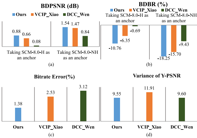
Fig. 8. Coding performance comparison between Ours and other popular rate control algorithms.
