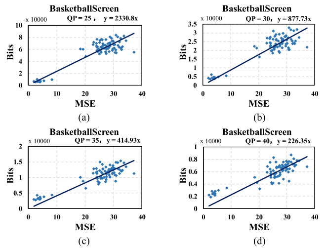
Fig. 6. The R-MSE curves for scene unchanged frames under different QPs.
