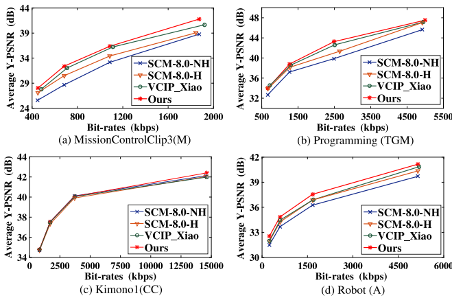
Fig. 10. R-D curves comparisons for different RC algorithms.
