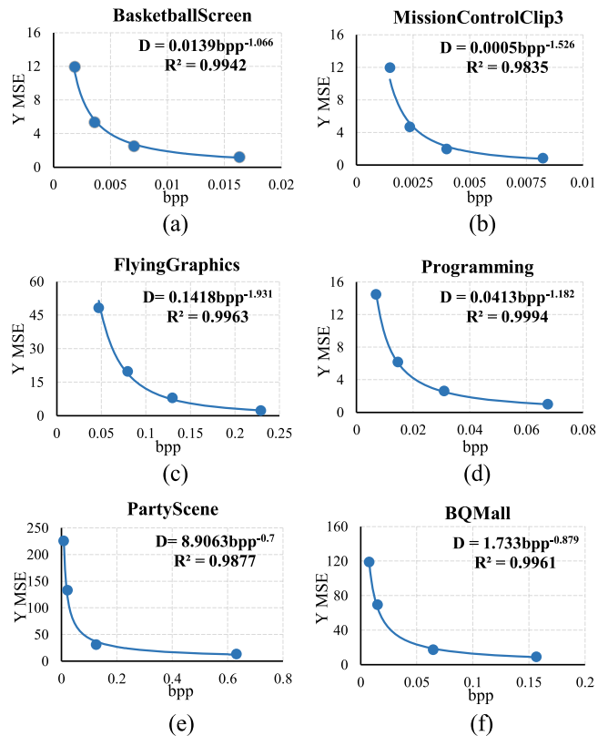
Fig. 2. R-D curves. (a), (b) mixed content videos; (c), (d) pure computer-generated content videos; (e), (f) pure camera-captured content videos.
