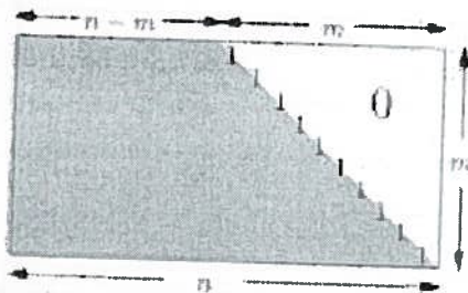
An equivalent parity-check matrix in lower triangular form.
