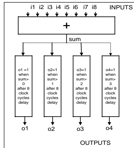
Figure 5: Behavior of the 8-input/4-output concentrator
