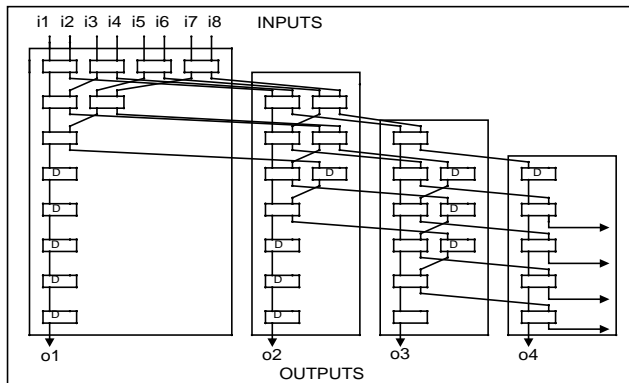
Figure 3: Structure of the 8-input/4-output concentrator
