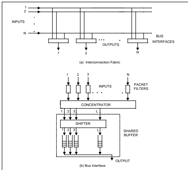
Figure 1: The Knockout ATM switch
