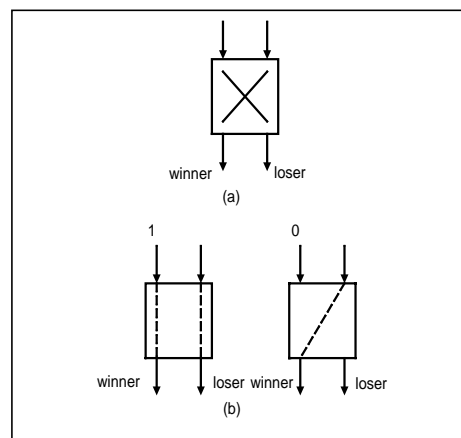
Figure 2: 2 \times 2 contention switch
