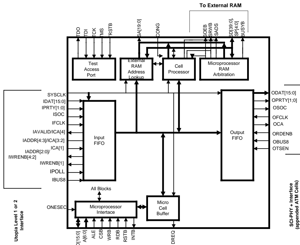
Figure 1. structure of the RCMP-800
