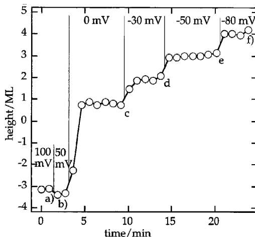
FIGURE 36.2 Height of the Cu nanostructure generated in a hole on a Au(111) surface as a function of time when a sequence of potential steps running in the negative direction are applied to the electrode. (From Xia et al., 1999, with permission from Elsevier.)
