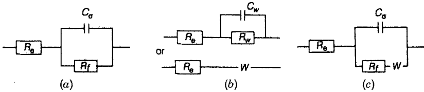
FIGURE 12.15 Electrode impedance with kinetic (a), diffusional (b), and combined (c) reaction control (W is the Warburg impedance).
