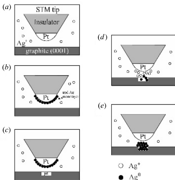
FIGURE 36.3 Schematic diagram illustrating the main features of the mechanism for STM-tip directed silver nanostructure deposition on graphite: (a) a freshly prepared polymer-coated platinum microelectrode is immersed in a dilute aqueous silver-plating solution, and a tunneling junction is established with a graphite basal plane surface; (b) silver is deposited at the underpotential on the Pt surface, resulting approximately in a silver atomic layer; (c) through application of a first bias pulse, a pit is formed on the surface of graphite; (d) Ag is desorbed from the tip through a second bias pulse; (e) a silver particle is formed on the pit by deposition of silver ions in its proximity. (From Li et al., 1996, with permission from the American Institute of Physics.)
