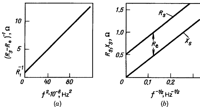
FIGURE 12.16 Examples for an extrapolation of experimental data to determine equivalent circuit parameters under kinetic (a) and diffusional (b) reaction control.
