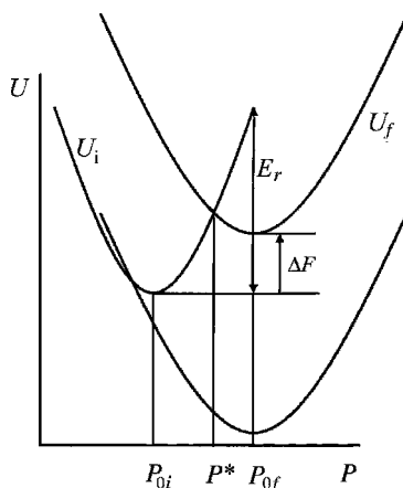
FIGURE 34.2 One-dimensional scheme of the free-energy surfaces of the initial and final states. Medium polarization plays the role of the reactive modes. Matching of the electron energy levels \varepsilon_D = \varepsilon_A corresponds to crossing of the free-energy surfaces U_i(\mathbf{P}^*) = U_f(\mathbf{P}^*) . Electron transfer corresponds to the transition from U_i to U_f at the transitional configuration \mathbf{P}^* . \Delta F is the free-energy of the transition. The lower free-energy surface of the final state corresponds to the inverted region.
