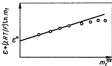
FIGURE 7.3 Extrapolation of experimental data for the determination of activity coefficients.
