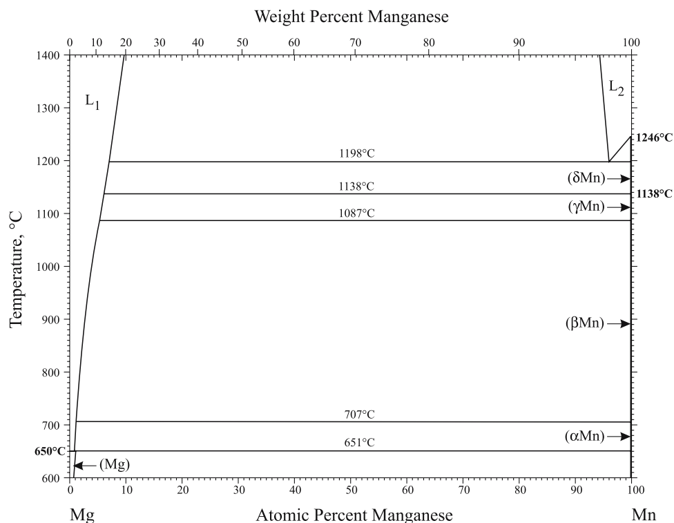
Fig. 1 Mg-Mn phase diagram
