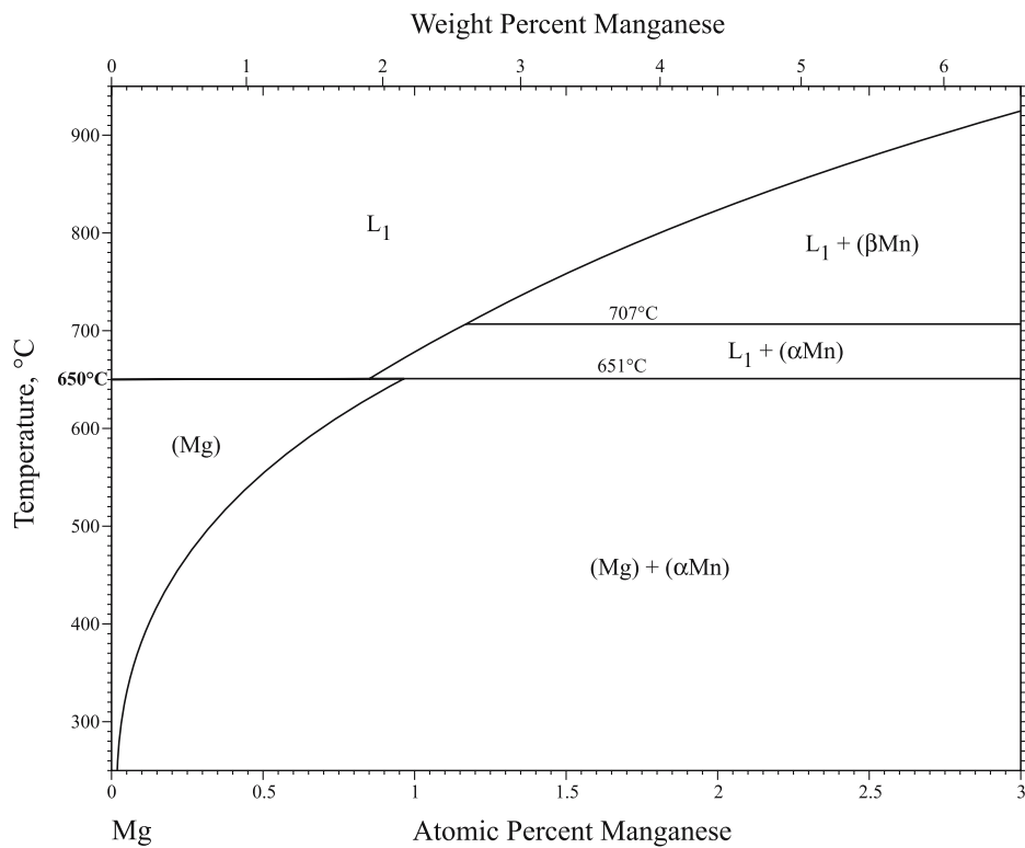
Fig. 2 Detail of Fig. 1 on the Mg-rich end
