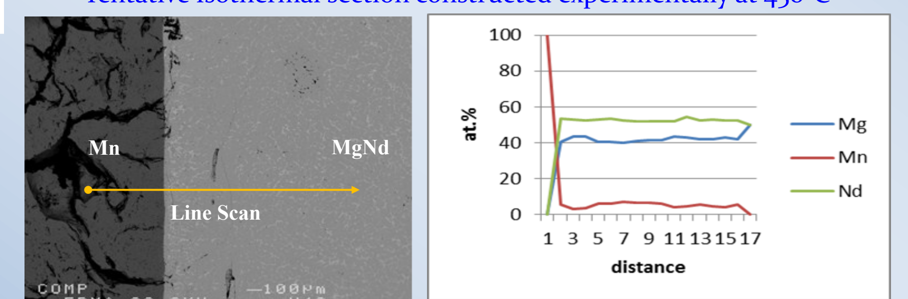
Diffusion couple from pure Mn to MgNd alloy annealed at 450°C and its composition profile
