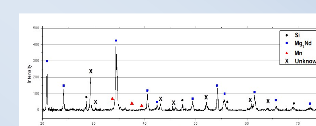
XRD spectrum and microstructure of sample # 1
