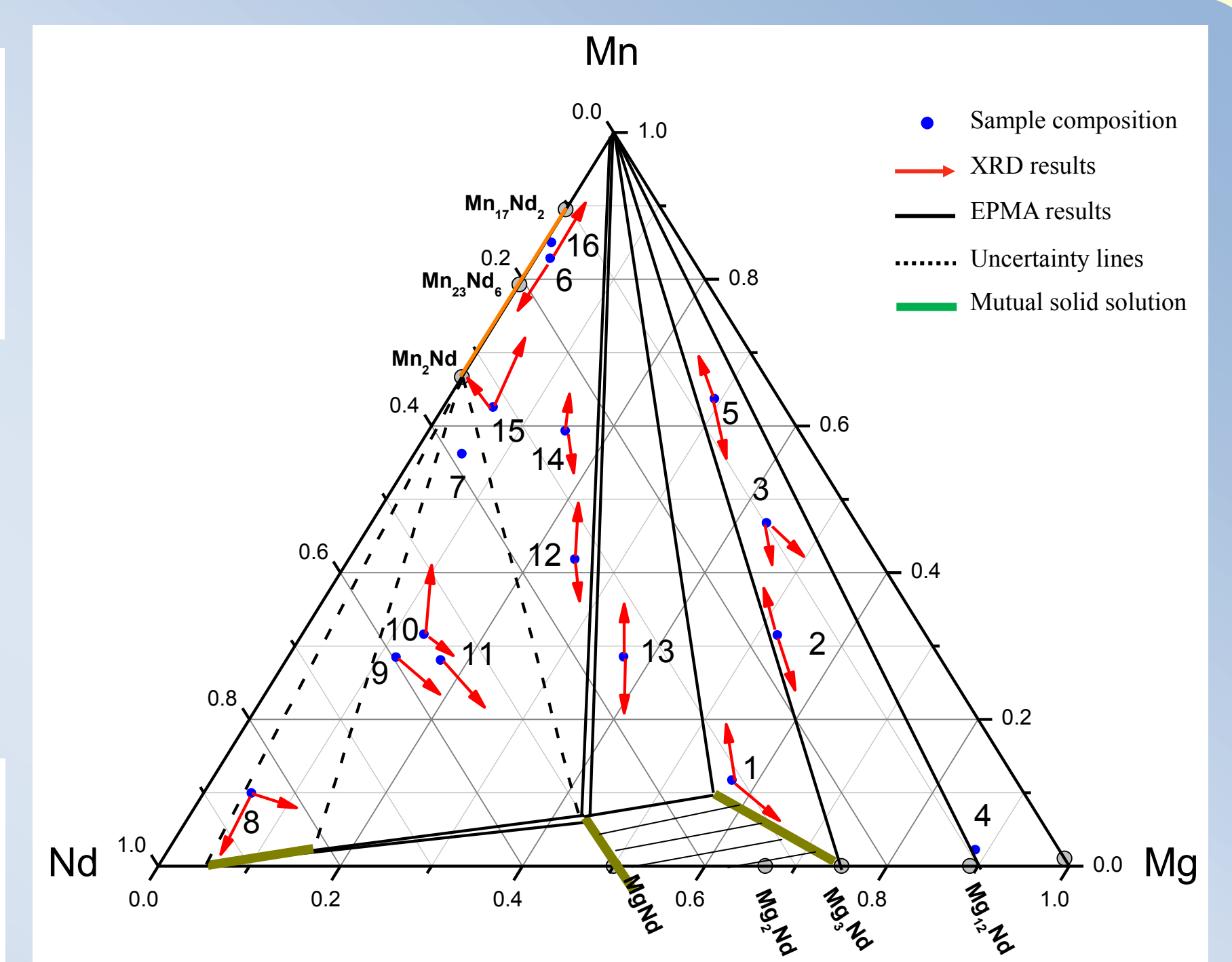
Tentative Isothermal section constructed experimentally at 450°C
