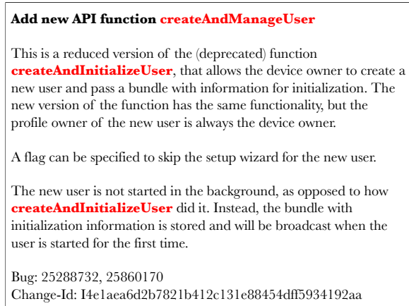
Figure 4: Android framework commit message 343fb33, presents a migration pathway.
