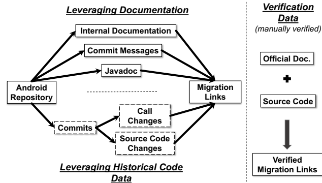
Figure 2: API migration extraction strategies.
