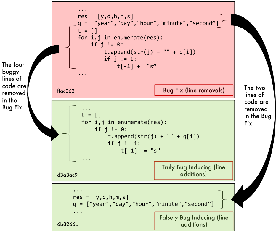
Fig. 5 Example of a bug-fix (ffac062) with two inducing commits, one bug-inducing (d3a3ac9), and one falsely bug-inducing (6b8266c)
