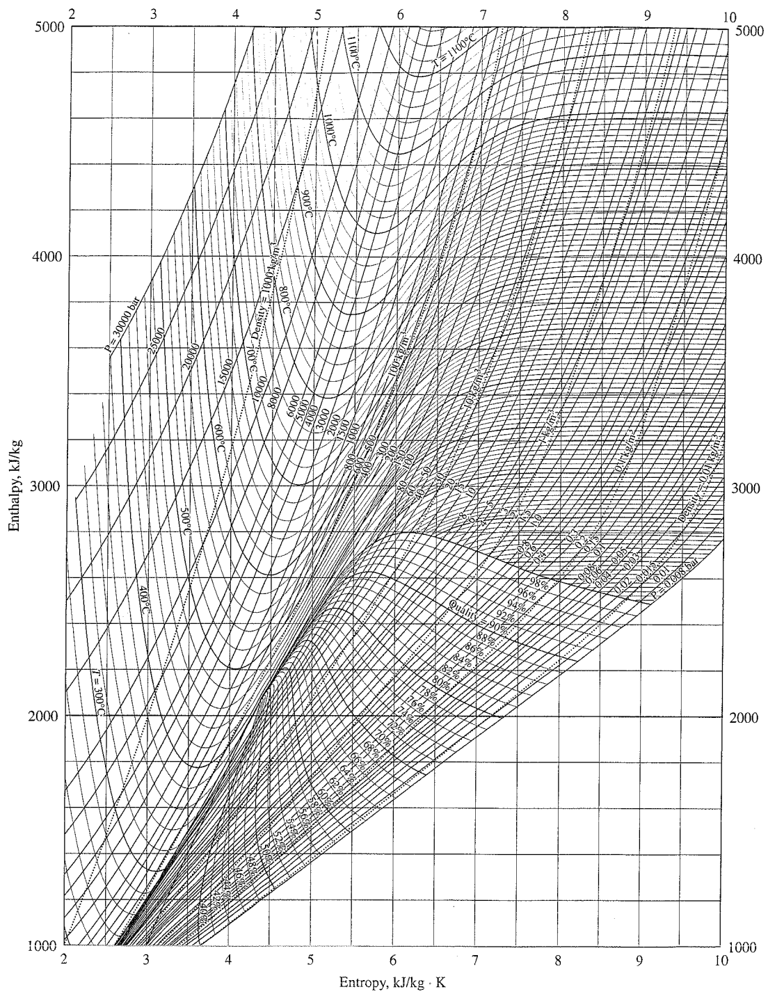
FIGURE A-10 Mollier diagram for water. (Source: Lester Haar, John S. Gallagher, and George S. Kell, NBS/NRC Steam Tables , 1984. With permission from Hemisphere Publishing Corporation, New York.)
