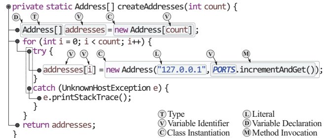
Figure 1: Representation of a method body as a tree.
