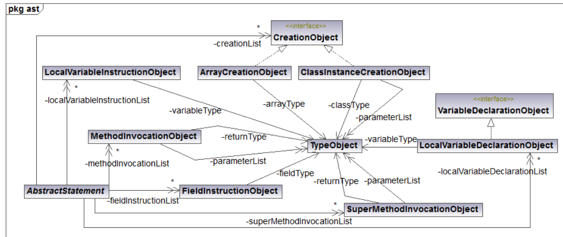
Figure 6.5: Representation of low-level Java elements.
