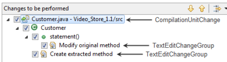
Figure 6.12: Representation of TextEditChangeGroups in a CompilationUnitChange .
