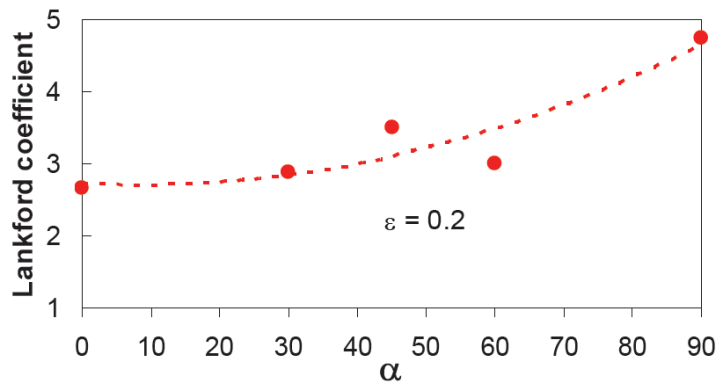
Figure 2: Lankford coefficient versus angle to rolling direction
