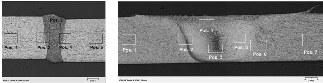
Fig. 6: Welded AZ31B joints a) laser beam welded, b) friction stir welded
