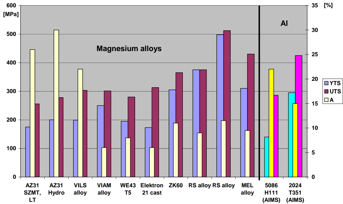
Fig. 1: Static properties of commercially available and new alloys.
