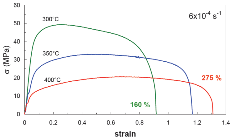
Figure 3: Tests at constant strain rate
