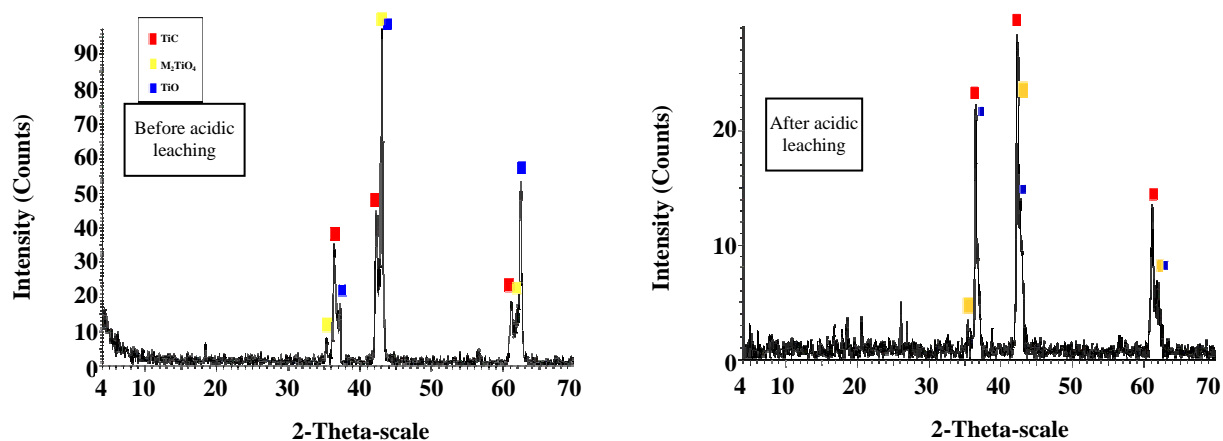
Fig. 5: XRD patterns of TiC before and after acidic leaching.
