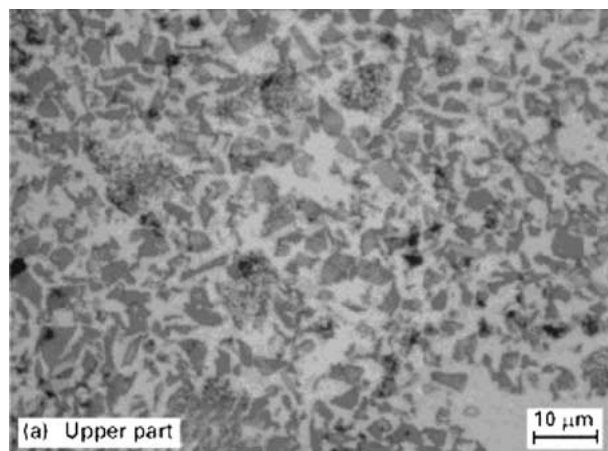
Figure 5 The microstructure of the infiltrated SiC/Mg composite [89].
