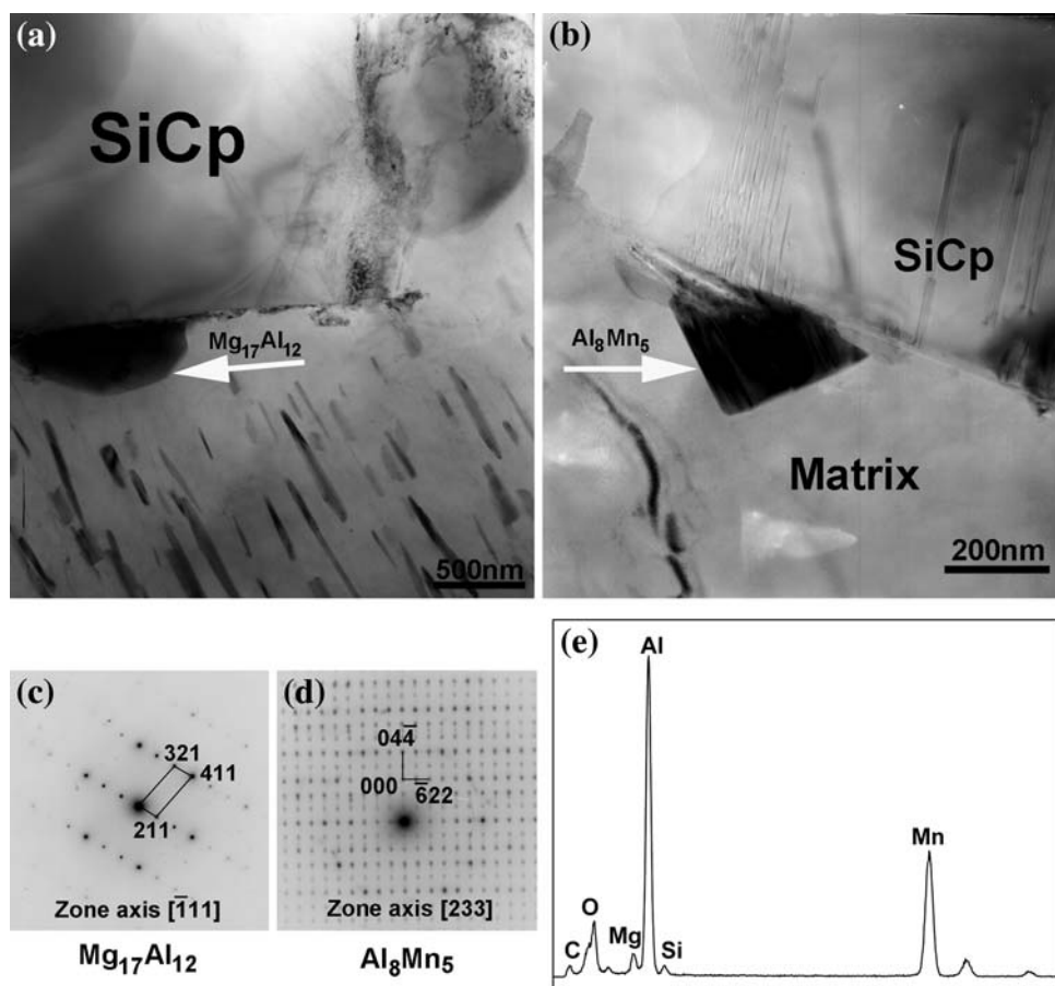
Fig. 4 Illustrating the presence of Mg_{17}Al_{12} and Al_8Mn_5 at the interface. a Mg_{17}Al_{12} ; b Al_8Mn_5 ; c and d are the corresponding electron diffraction patterns for Mg_{17}Al_{12} and Al_8Mn_5 in (a) and (b), respectively; e corresponding EDAX spectrum for Al_8Mn_5 in (b)
