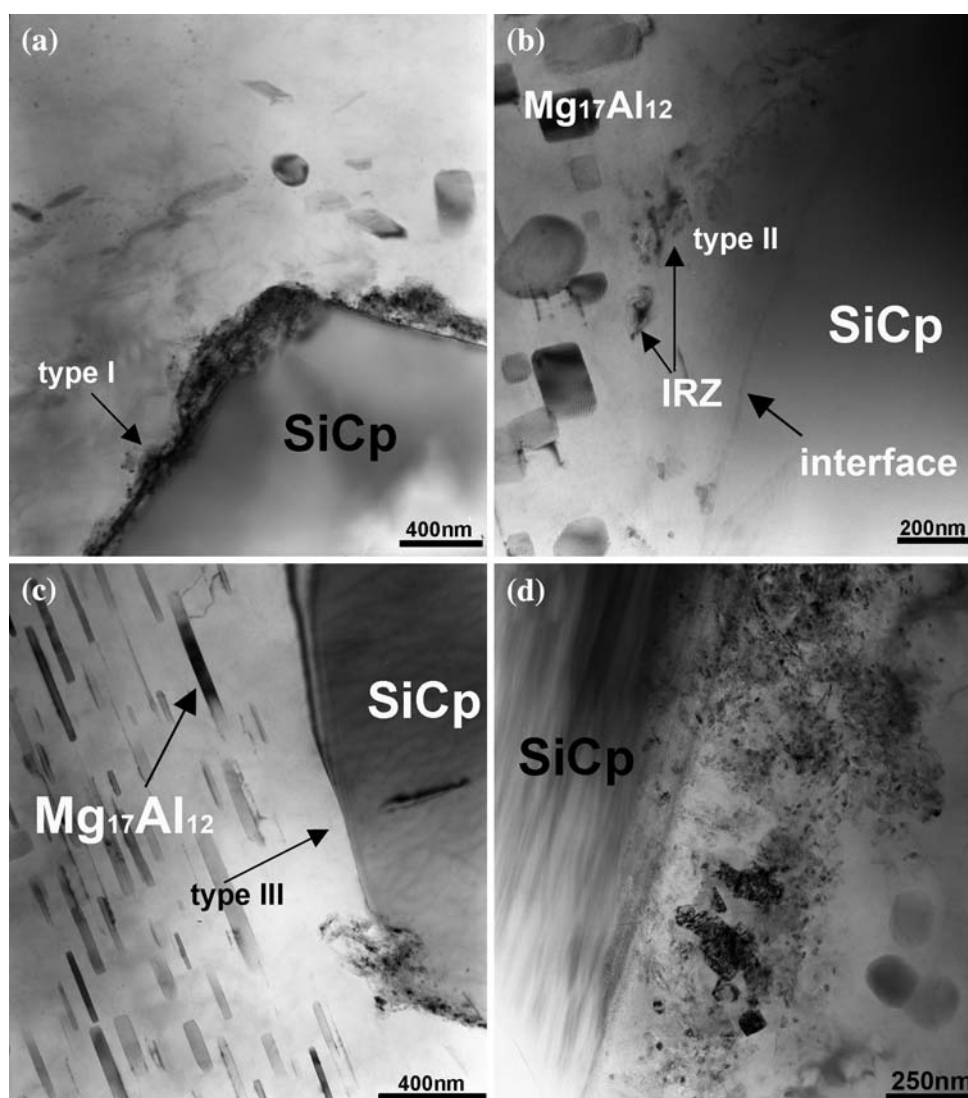
Fig. 1 TEM morphologies of the three distinct interfaces between SiCp and matrix. a interface I; b interface II; c interface III; d morphology of IRPs at interface I
